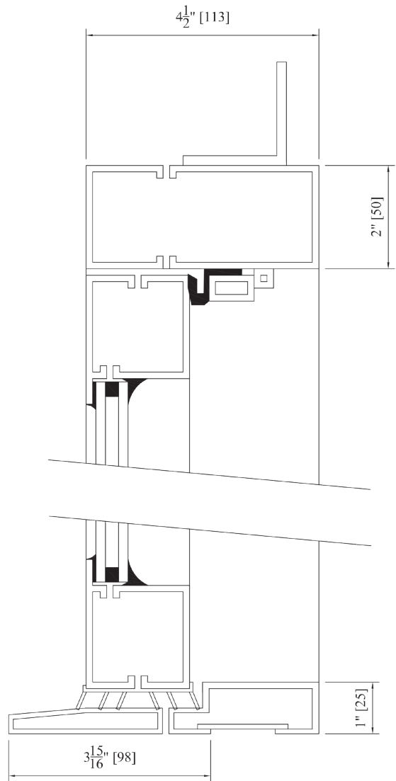
Standard Jamb and sill Profile Swing Out
