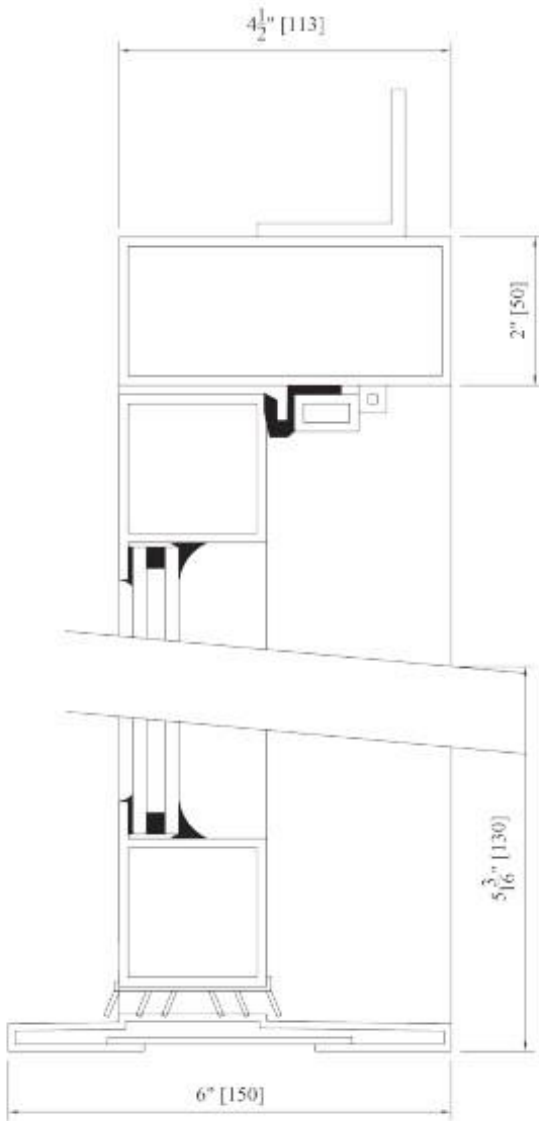
Standard Jamb and ADA sill Profile Swing Out
