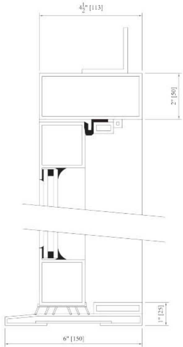
Standard Jamb and sill Profile Swing Out
