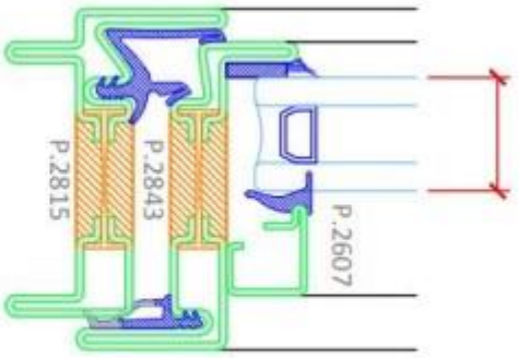
Horizontal Pivot Window- Top
