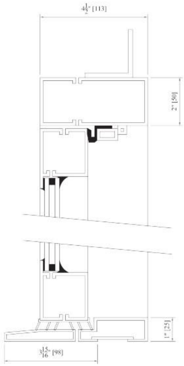
Standard Jamb and sill Profile Swing Out
