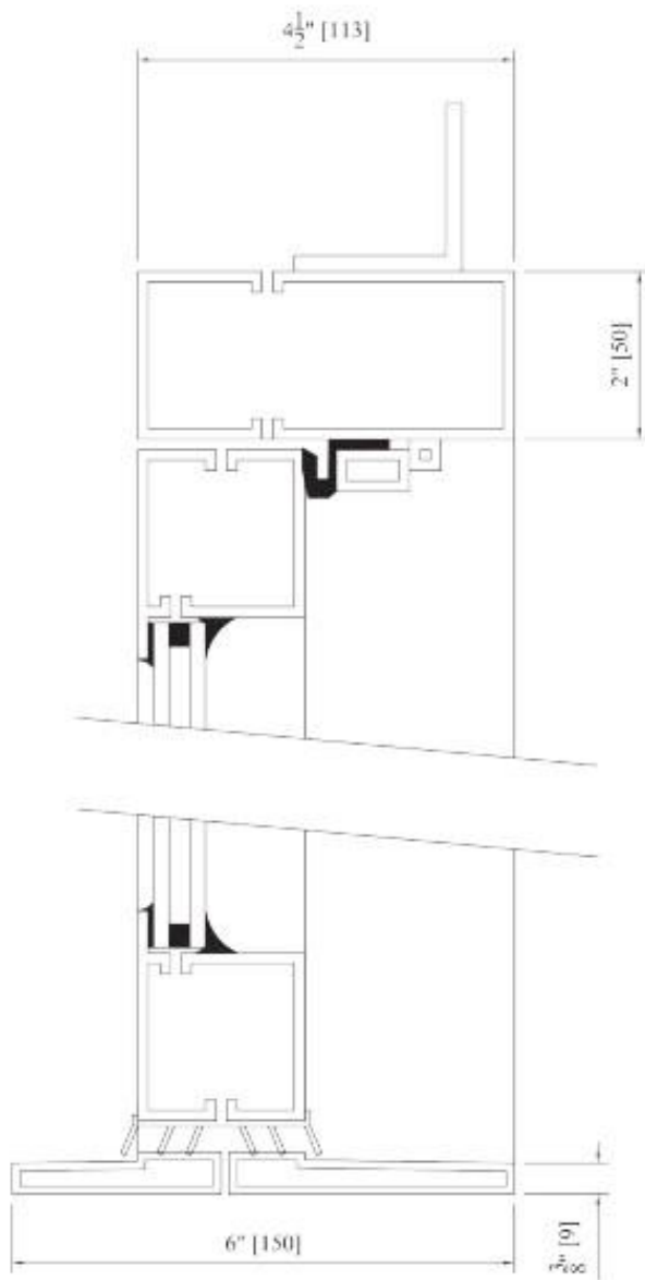
Standard Jamb and ADA sill Profile Swing Out
